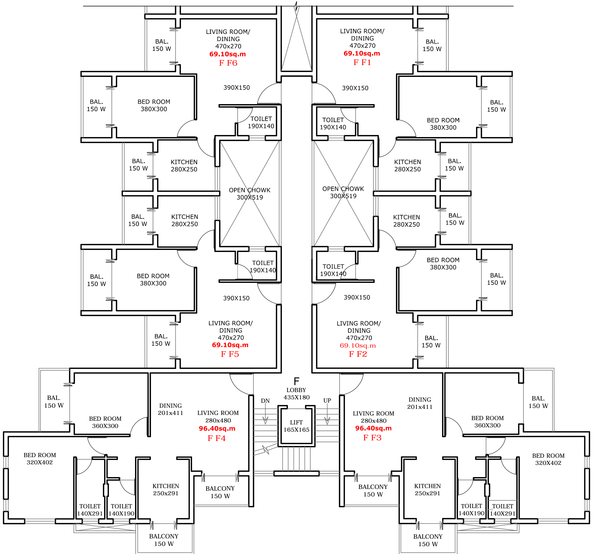
FIRST FLOOR PLAN BUILDING EF - PART F
