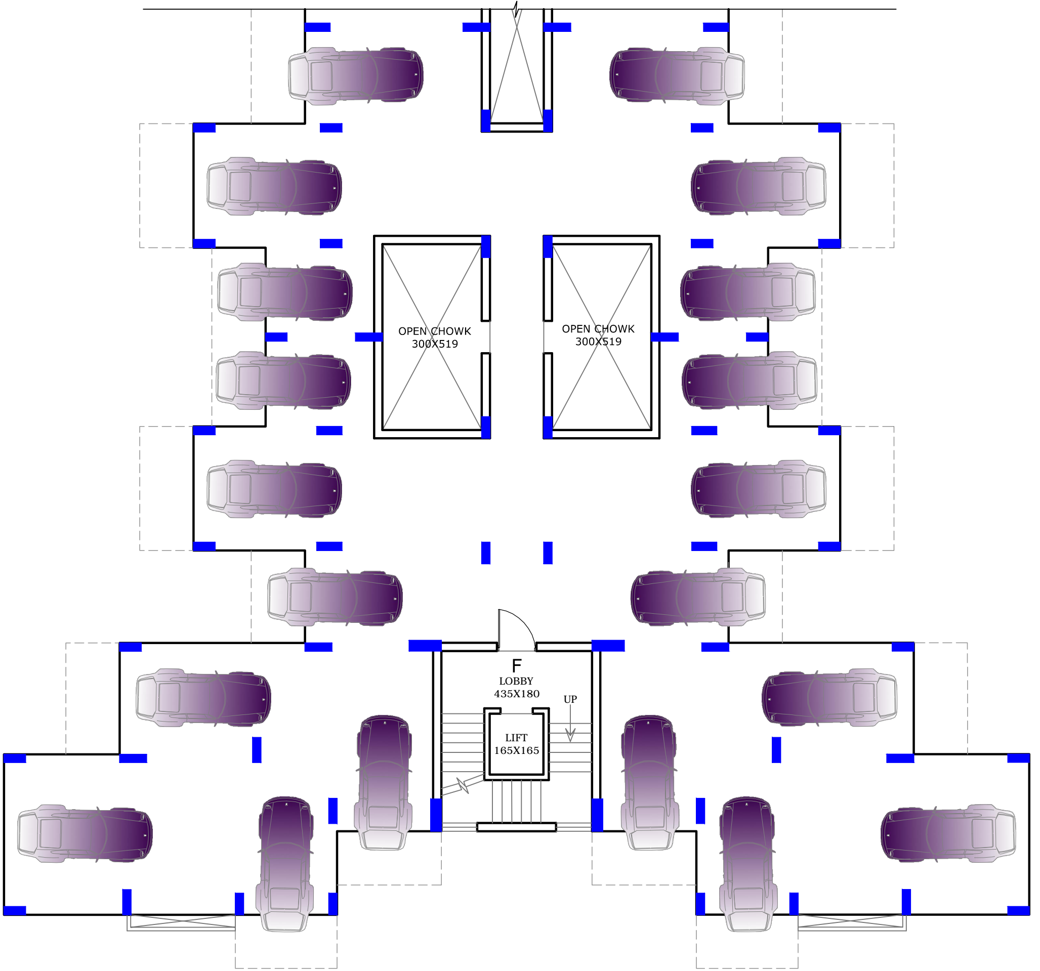
STILT FLOOR PLAN BUILDING EF - PART F
